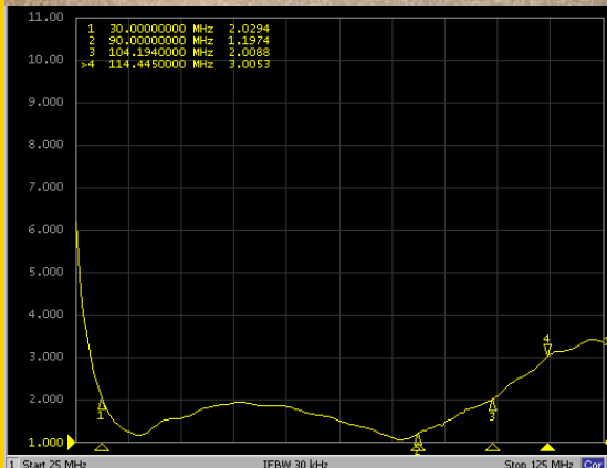
Measured VSWR over 25-125 MHz range
